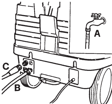
Raccordement hydraulique.
